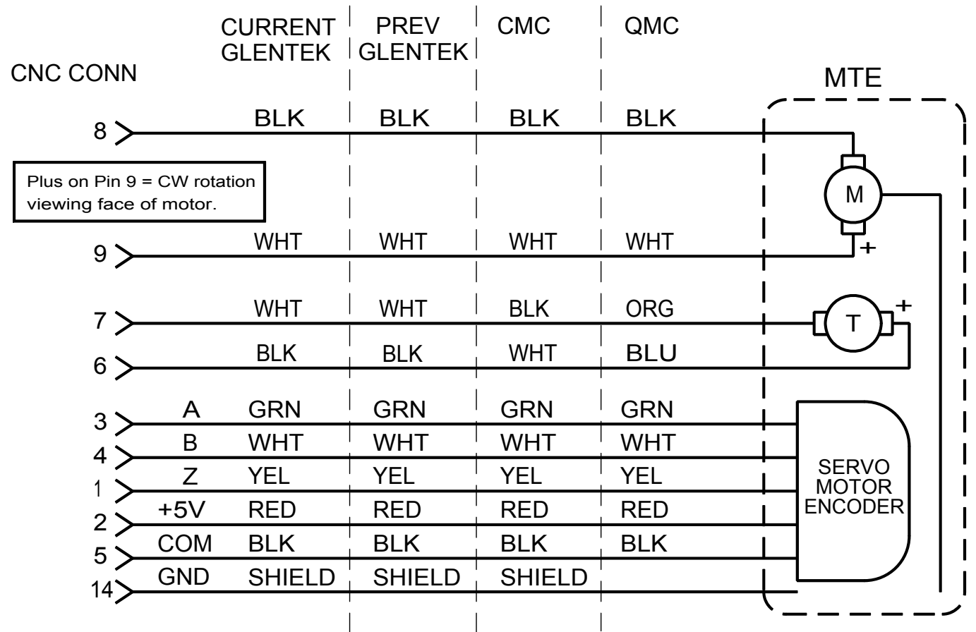
MTE_servo_encoder_wiring.dcd
