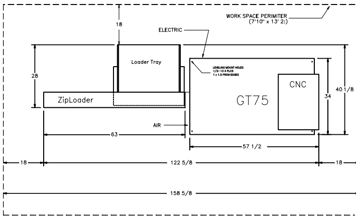
PLAN VIEW: GT75 w/ZipLoader
