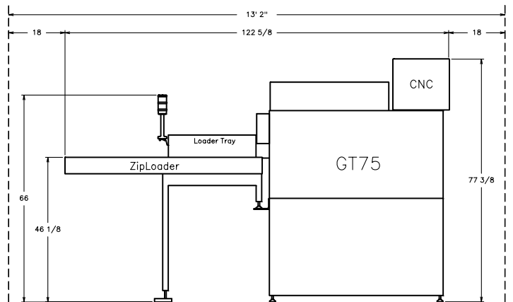
FRONT VIEW: GT75 w/ZipLoader
